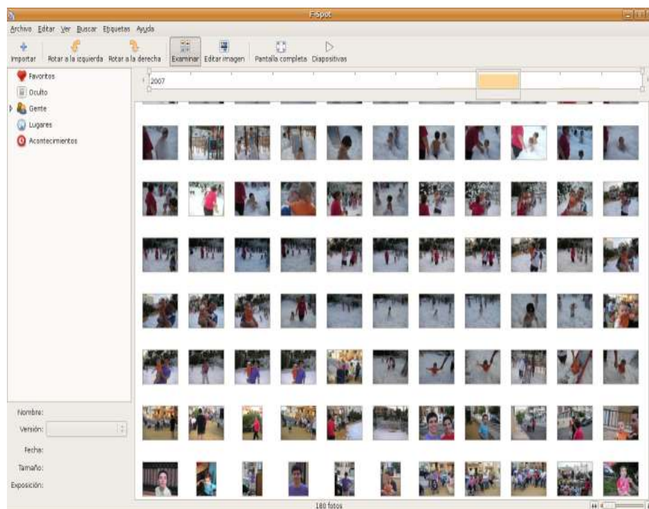
Interfaz principal
