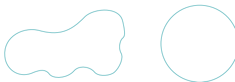
closed curves
