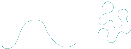
open curves
