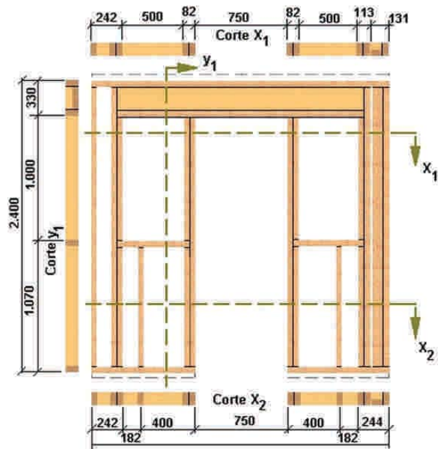
Figura 10–70: Tabique perimetral TSP p2v4 -2400x2360-(1).
